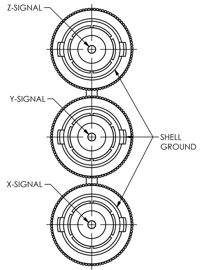
BNC PINOUTS SCALE 2.5X
