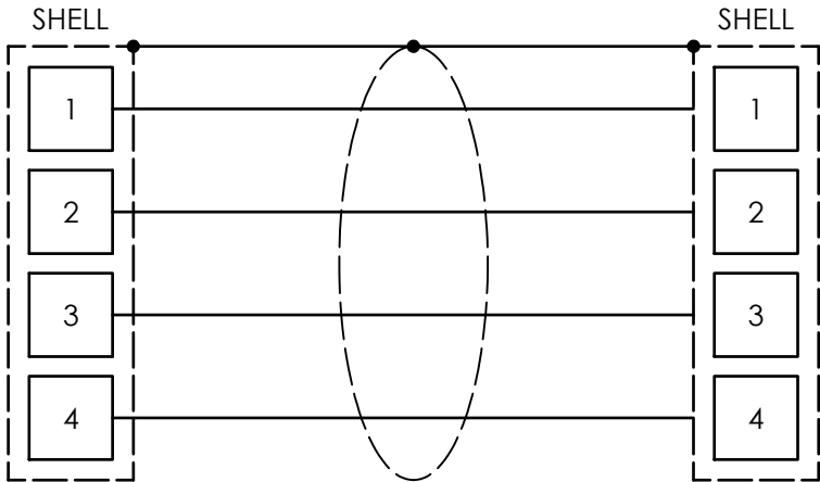
SCHEMATIC DIAGRAM
