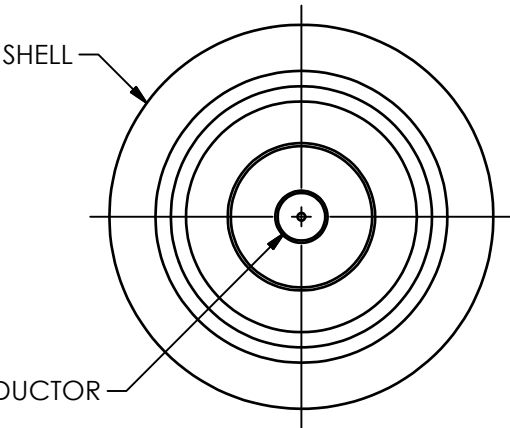
023-FZ- PINOUT SCALE 8X
