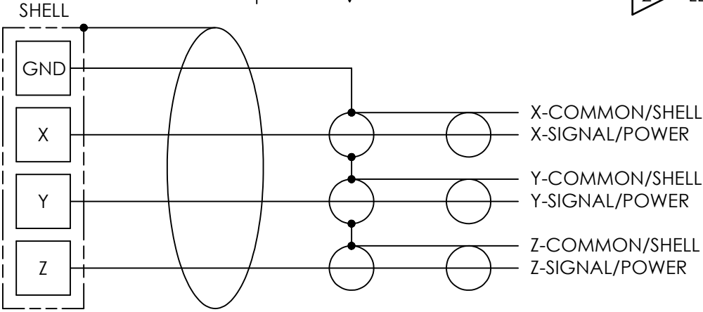
SCHEMATIC DIAGRAM
