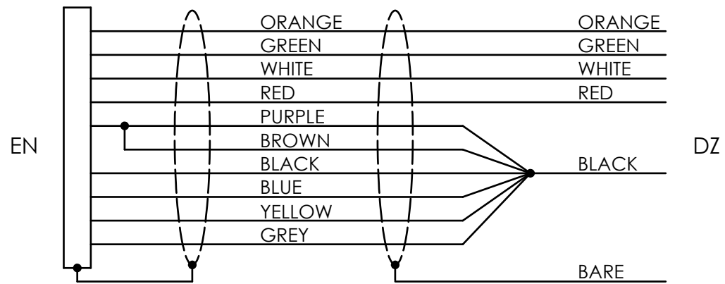
SCHMATIC DIAGRAM (M)037ENDZ-XXXX CABLES AND 037PXX SERIES 30' [10] AND UNDER
