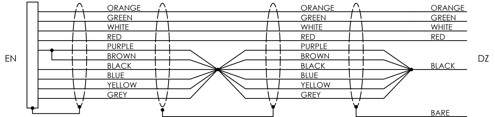
SCHMATIC DIAGRAM (M)037ENDZ-XXXX CABLES AND 037PXX SERIES CABLES OVER 30' [10]
