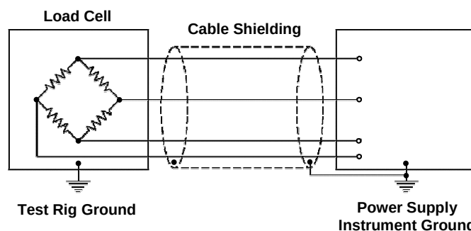
Figure 5 - Grounding
