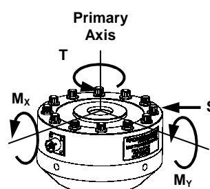
Figure 13 - Extraneous Loads
