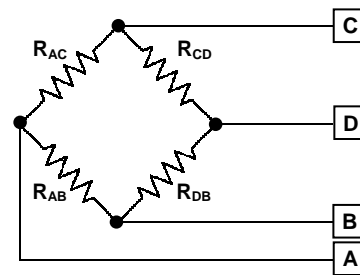
Figure 17 – Wheatstone Bridge
