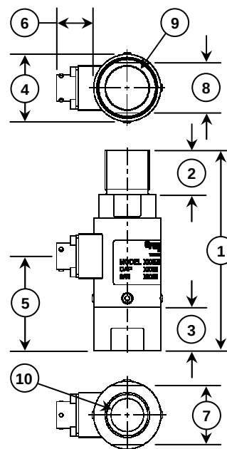
Figure 2 - Dimensions
