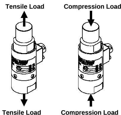
Figure 1 - Rod End Load Cell Loads
