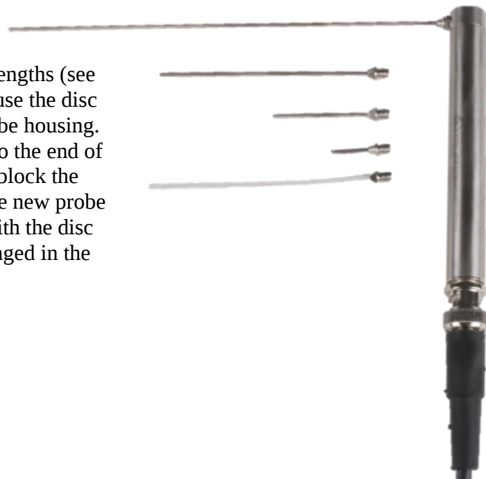
Figure 4: Probe Tips
