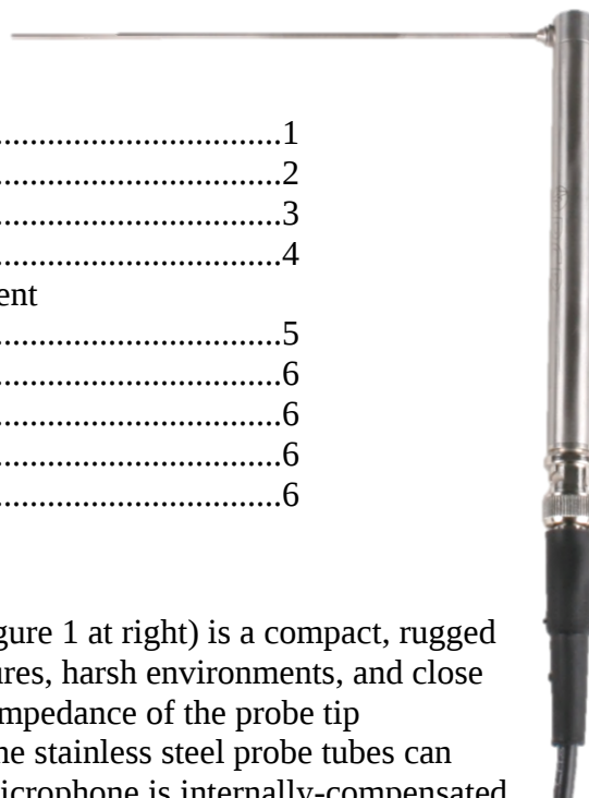
Figure 1: 377B26 Probe Microphone
