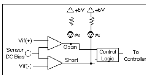
Figure 3 Input Fault Window Comparator with LED Indicator
