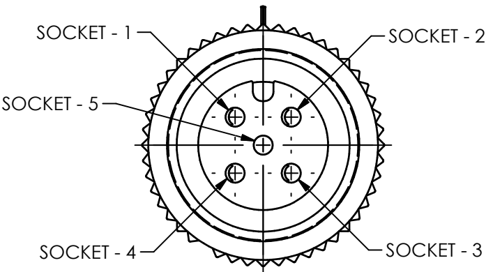
5-SOCKET, M12 (FEMALE) CONNECTOR SCALE 3X
