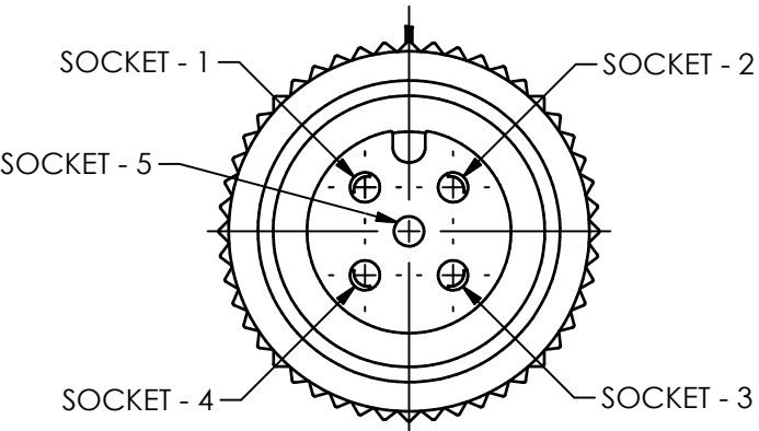
5-SOCKET, M12 (FEMALE) CONNECTOR SCALE 3X
