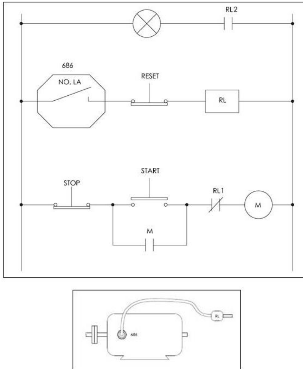
Figures 17 and 18 – Automatic Machinery Shutdown Using an External Electromechanical Relay
