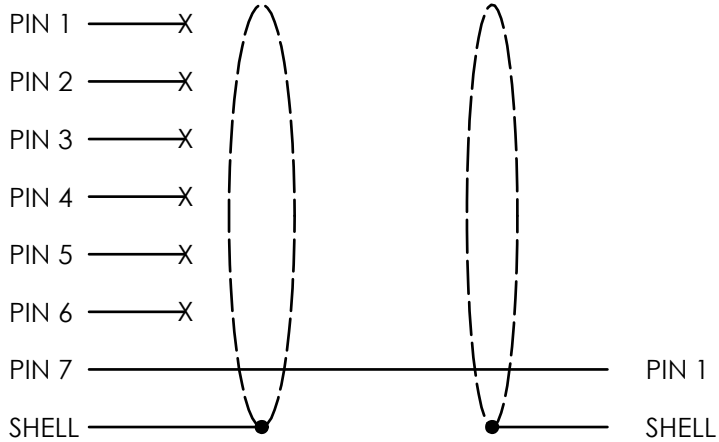
SCHEMATIC DIAGRAM
